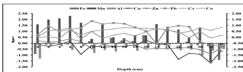
Fig. 6. Geo-accumulation (Igeo) for major elements and trace metals in cores collected from Kushavati river (a) and Zuari river (b) of Goa, West-coast of India.
