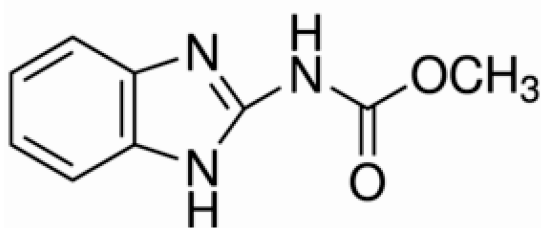
Fig. 1. Molecular structure of carbendazim.
