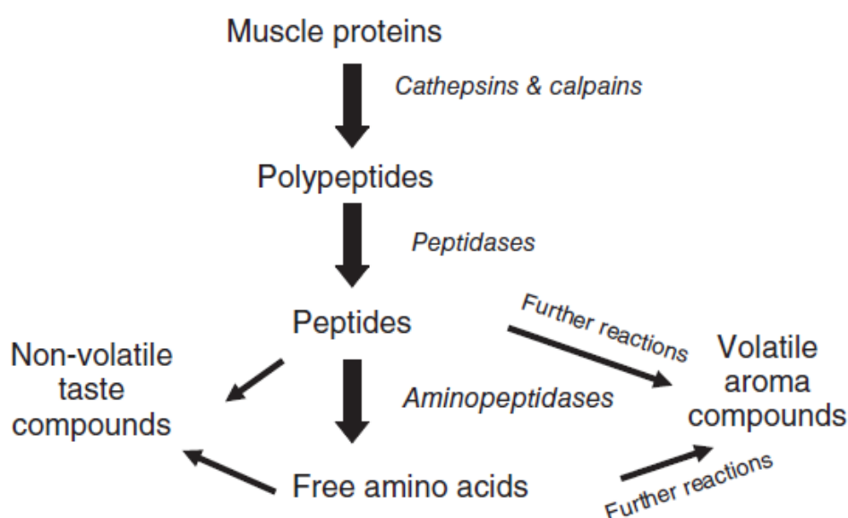
Figure 6 - Meat protein
