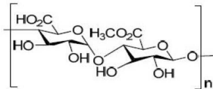
Figure 5 - Pectin structure
