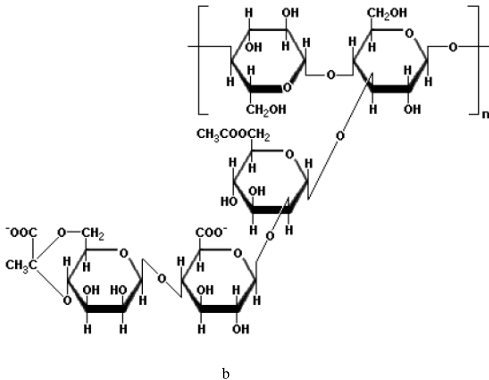
Figure 4- Hemicellulose structure
