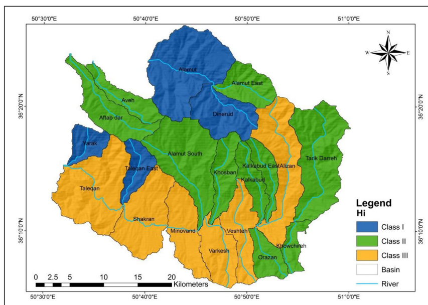
Fig. 2. Spatial distribution of Hi values.
