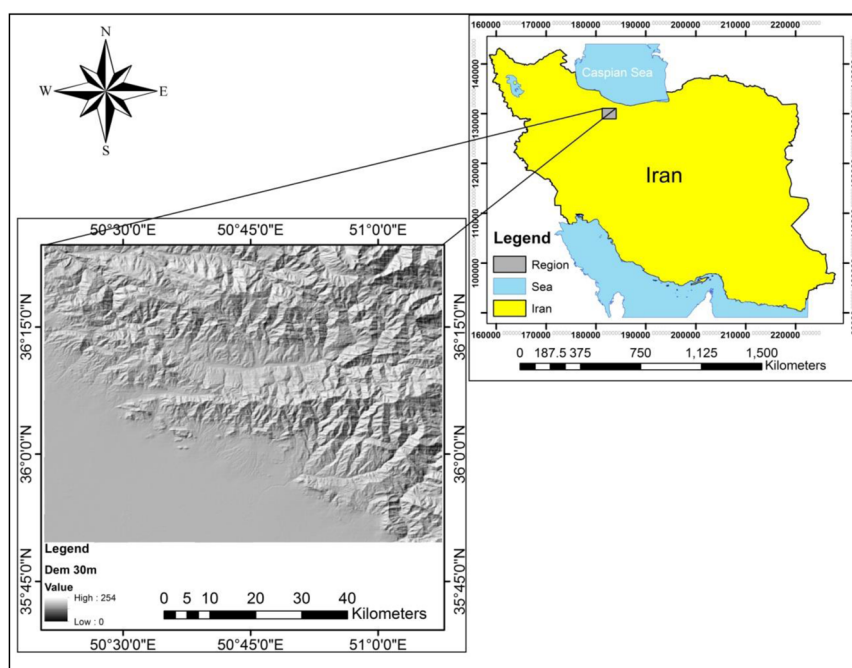
Fig. 1. Location of the study area on the map of Iran (data extracted from digital maps of the Organization of Geological Survey and Mineral Exploration of the country).
