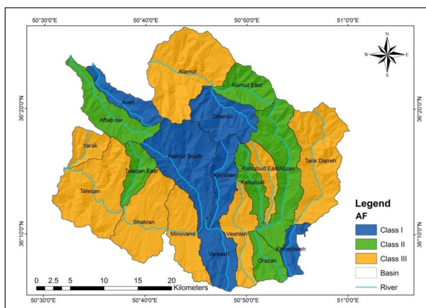
Fig. 3. Spatial distribution of AF values.
