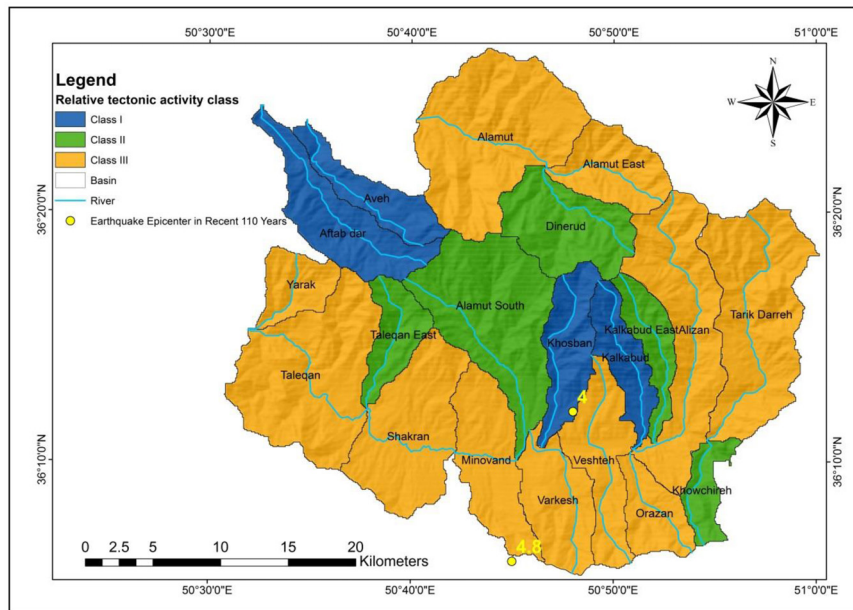
Fig. 7. The distribution map of the center of earthquakes in the recent 110 years in the study area.
