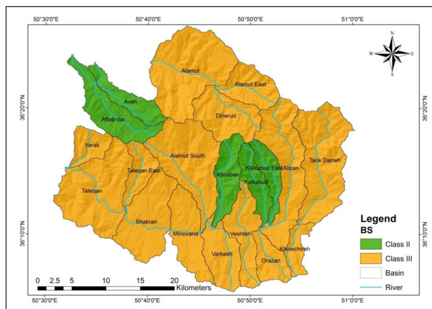
Fig. 4. Spatial distribution of Bs index values.
