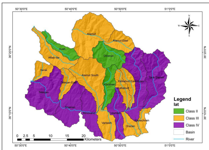
Fig. 5. Relative tectonic activity classes (I at) by color.
