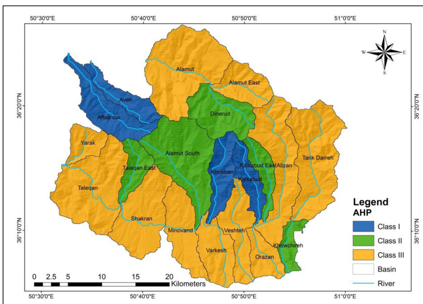
Fig. 6. The relative tectonic activity categories using Analytical Hierarchy Process (AHP).
